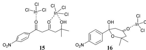
Fig. 4 Possible intermediates 15 and 16 implicated in rate reduction.
