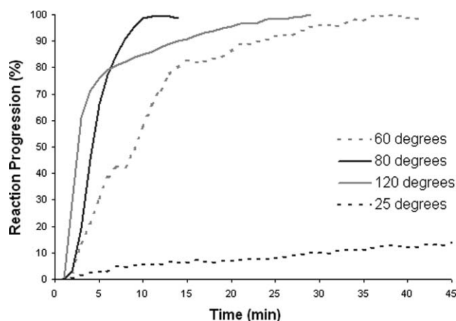
Fig. 2 Rate of change in IR spectra for transformation of diketone 3 into pyran-4-one dependent on reaction temperature.
