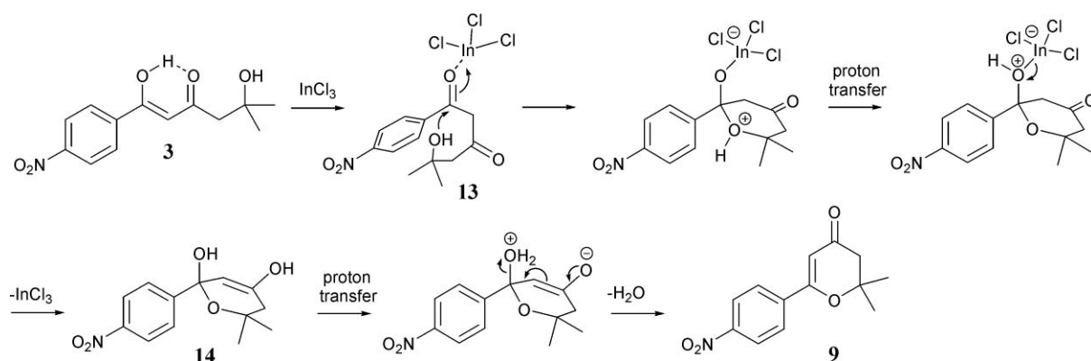
Scheme 3 Proposed mechanism of pyran-4-one formation.
