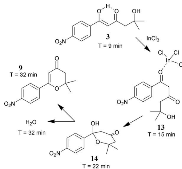
Scheme 2 Species observed by in situ IR spectroscopy.
