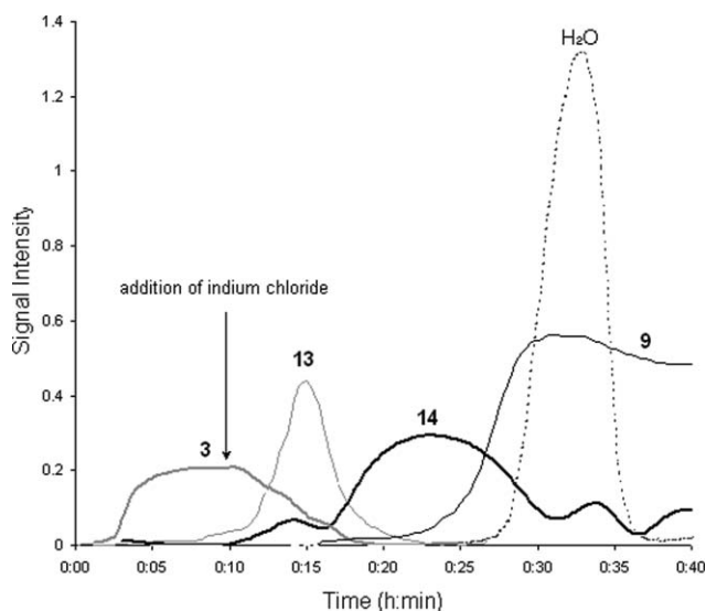
Fig. 3 Identified reaction components (compounds 3 , 9 , 13 and 14 ) as a function of time.
