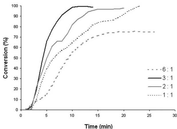
Fig. 1 Rate of change in IR spectra for transformation of diketone 3 into pyran-4-one dependent on diketone : \text{InCl}_3 ratio. Reaction conditions: 0.055 M toluene solution of 3 maintained at 80 °C.
